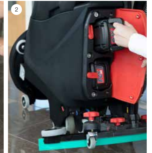
1 TTB1840NX Battery Replacement
